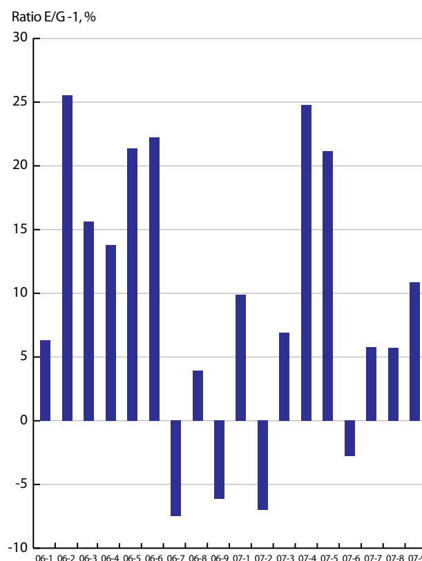
Figure 4.9. Comparison of total lipid results obtained from gravimetric and enzymatic methods.
