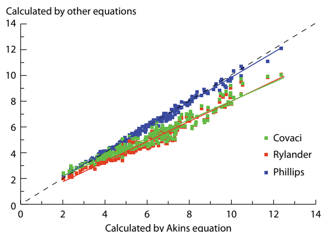
Figure 4.10. Calculation of total lipids in serum from enzymatic data.
