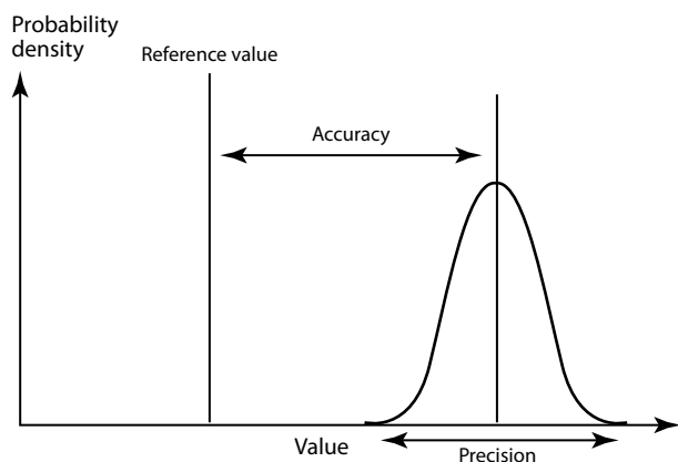
Figure 4-1. Comparison of precision and accuracy.
