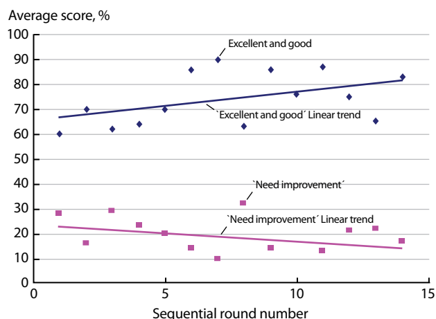
Figure 4-11. Performance trends for POPs 2002 to 2006.
