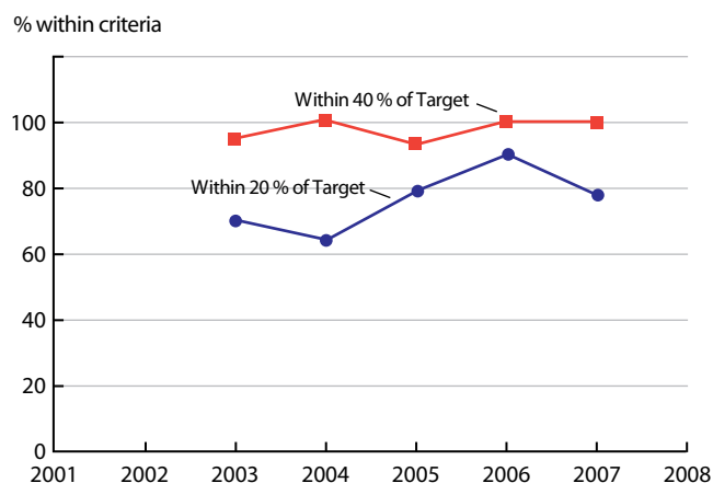
Figure 4.7. Lipid analysis performance over time. Data from all participants are plotted.
