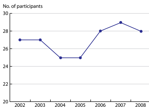
Figure 4.2. Trend in participation in the AMAP Ring-tests.
