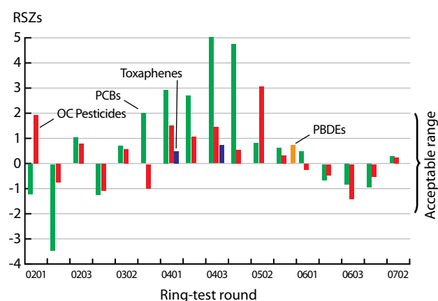
Figure 4.5. An individual participant's performance using RSZs.
