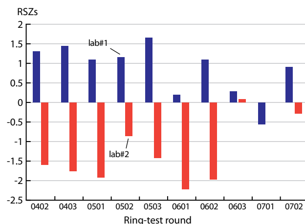
Figure 4.8. A comparison of lipid results for two laboratories.
