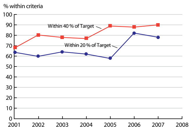
Figure 4.3. Performance trends for individual analytes: CB28. Data from all participants are plotted.
