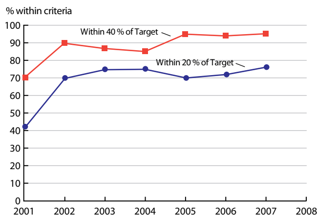
Figure 4.4. Performance trends for individual analytes: CB138. Data from all participants are plotted.
