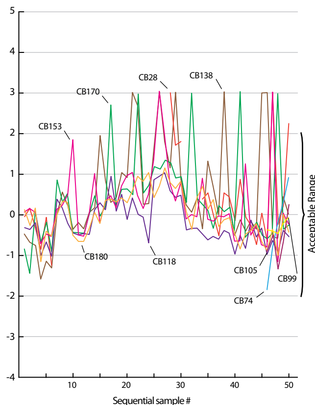
Figure 4.6. Individual PCB congener performance over time.
