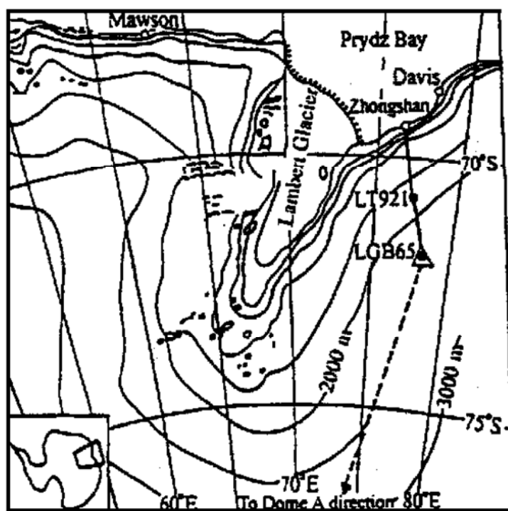
Fig. 1. Map showing the route of the Chinese First Antarctic Inland Traverse during 1996/1997. ● : the location of the two snowpits; △: the location of the firn.
