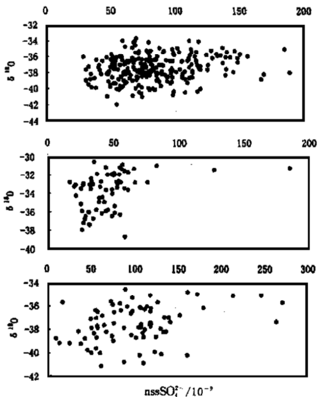
Fig. 4. The relationship between \text{nssSO}_4^{2-} concentration and \delta^{18}\text{O} in 50 m firn core and two snow pits. Up: 50 m firn core; Middle: LT921 snow pit; Down: LGB65 snow pit.
