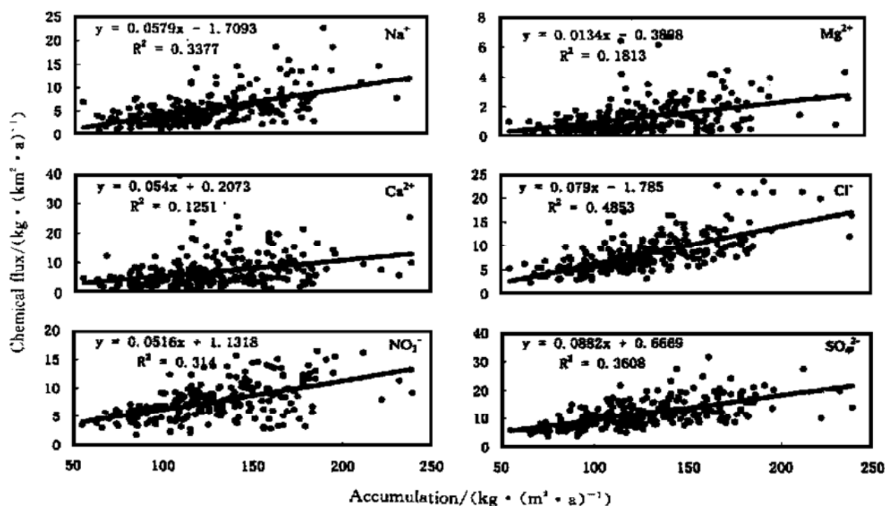
Fig. 3. The relationship between the chemical flux ( \text{Na}^+ , \text{Mg}^{2+} , \text{Ca}^{2+} , \text{Cl}^- , \text{NO}_3^- and \text{SO}_4^{2-} ) and the snow accumulation rate in the 50 m firn core. The solid line denotes the monistic linear regression curve. The formula in the upper part of left-hand side represents the regression one.
