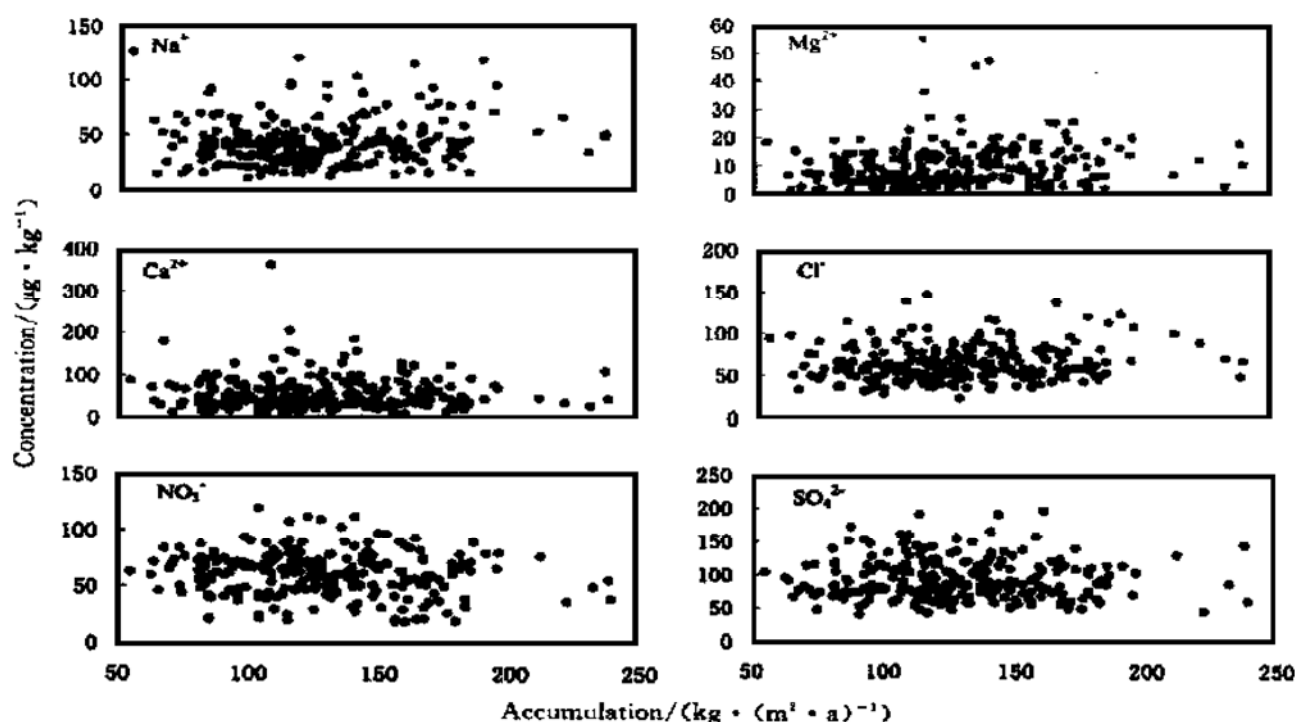
Fig. 2. The relationship between the chemical concentration ( \text{Na}^+ , \text{Mg}^{2+} , \text{Ca}^{2+} , \text{Cl}^- , \text{NO}_3^- and \text{SO}_4^{2-} ) and the snow accumulation rate in the 50 m firn core.
