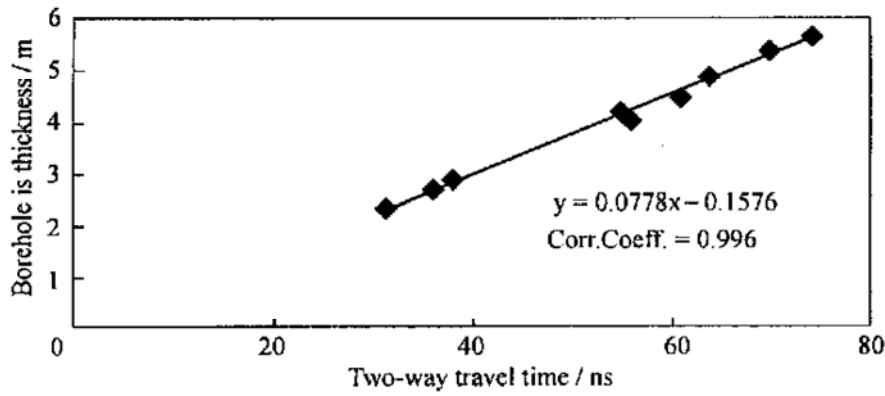
Fig. 3. Relationship between two way travel time and sea ice thickness.
