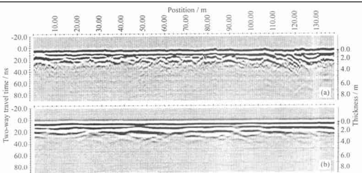
Fig. 4. Comparison of morphology of Arctic Summer sea ice bottom surface (a) is multi-year ice, (b) is first-year ice.
