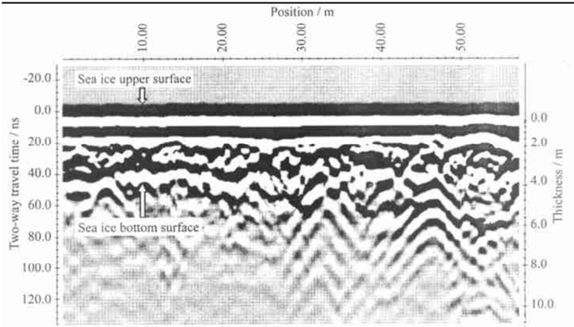
Fig. 2. A section of radar penetration survey profile from Arctic sea ice
