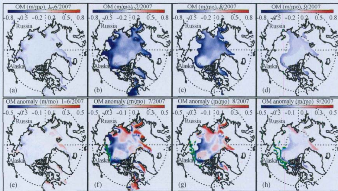
Fig. 11 Simulated ocean heat induced ice melting (OM) (a-d) and anomaly (e-h). Green line is the 2.0 \text{MJm}^{-2}\text{mo}^{-1} contour of the simulated ocean heat convergence anomaly plotted in Figure 10. The black circle marks the location of an ice mass balance buoy deployed in the Beaufort Sea during summer 2007 [29] .
