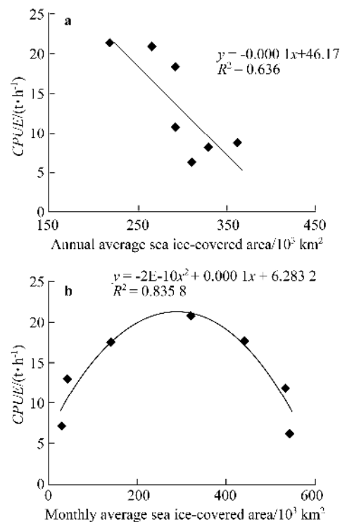
Figure 5 Linear (a) and polynomial (b) relationship between sea ice-covered area and CPUE.
