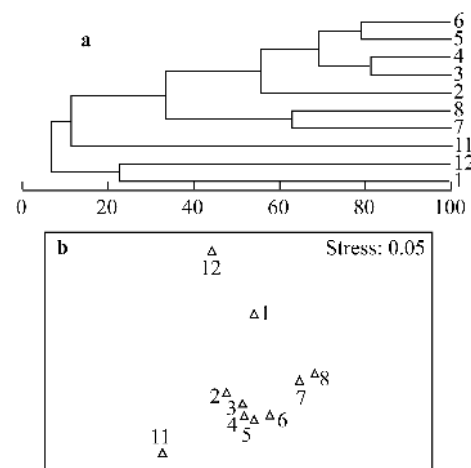
Figure 3 Cluster analysis (a) and nMDS ordination plot (b) of catches between fishing months according to the Bray-Curtis similarity. The stress value is given in the top right-hand corner of the ordination plot.
