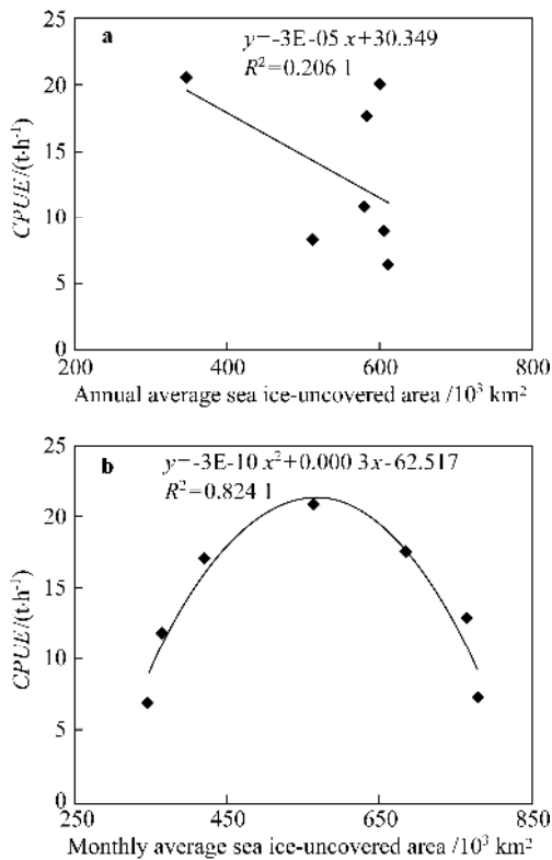
Figure 8 Linear (a) and polynomial (b) relationship between sea ice-free area ( -2^{\circ}\text{C} \leq \text{SST} < 3^{\circ}\text{C} ) and CPUE .
