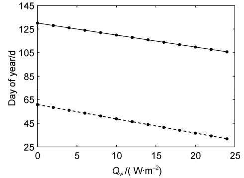
Figure 6 The times (in Julian days) when the modelled ice thickness reached the seasonal maximum value (broken line) and the modelled breakup date (solid line) versus different Q_w in Lake Wuliangsuhai with a thin snow cover on top.
