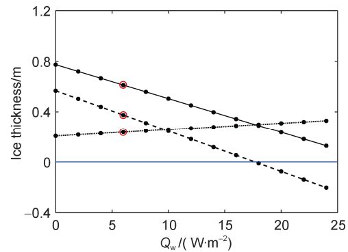
Figure 9 The modelled maximum lake ice thickness (solid line), congelation ice (broken line) and granular ice (dashed line) as a function of Q_w applied for the model runs in Lake Orajärvi. The red circle on each line is the validation experiment result. The black dots are Q_w applied in model experiments. The zero-reference level is the blue line.
