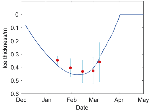
Figure 4 Modelled ice thickness evolution using constant Q_w = 14 \text{ W}\cdot\text{m}^{-2} in Lake Wuliangsuhai during the simulation period. The red dots are the observed 15-day multi-seasonal mean ice thickness. The vertical bars show the standard deviations.
