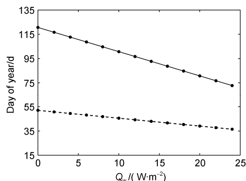
Figure 3 The times (Day of year) when the modelled ice thickness reached the seasonal maximum value (broken line) and the modelled breakup date (solid line) versus Q_w in Lake Wuliangsuhai.
